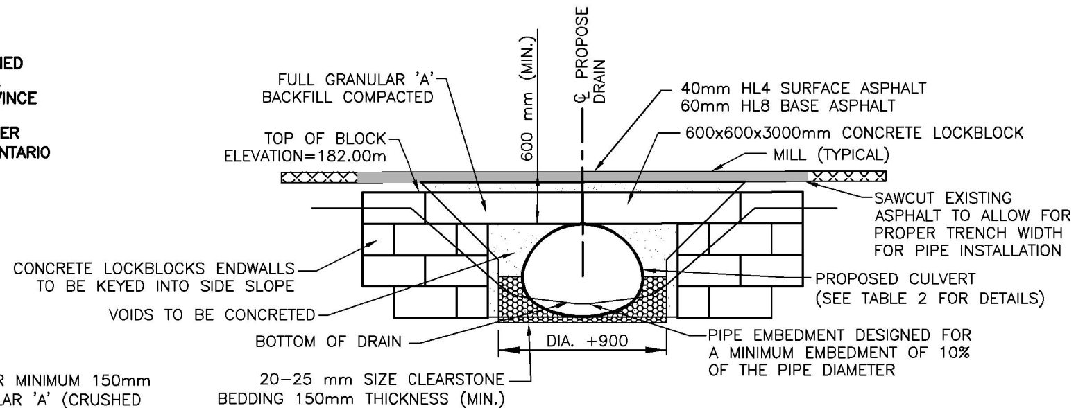
ROAD BRIDGE CROSS SECTION BRIDGE NO. 13 NOT TO SCALE
